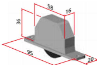
art. 2285 Carrello a pavimento con ruota rivestita in gomma Lower carriage with spring and wheel covered with rubber
