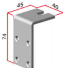
art. 2226 Staffa a "L" (interasse 36mm) per fissaggio pannelli in trucioare Strap at "L" (wheel base 36mm) or the fixing of chipboard panels
