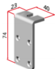
art. 2224 Staffa a "L" (interasse 13mm) per fissaggio pannelli in trucioare Strap at "L" (wheel base 13mm) or the fixing of chipboard panels
