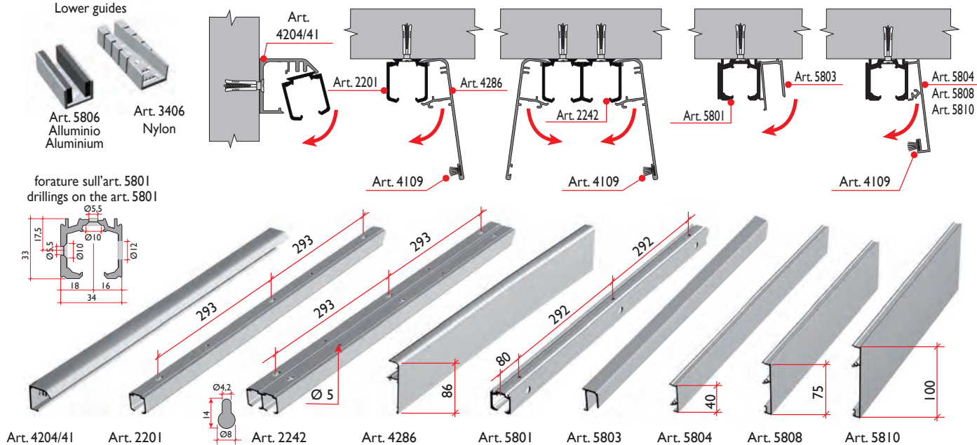
Guide inferiori Lower guides
