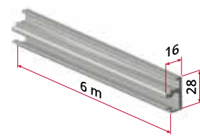
art. 2235 Profilo in alluminio per ancoraggio binario art. 2235 Aluminium profile for hooking the rail art. 2235
