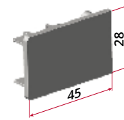
art. 2232/5 Tappo in plastica per art. 2231+2235 Plastic cap for art. 2231+2235
