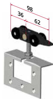
art. 2203/38 60* Carrello in nylon regolabile completo di staffa art. 2238 Nylon carriage adjustable with metal bracket art. 2238
