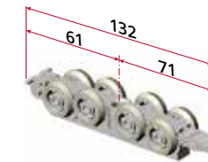
art. C/ACC8R 160* Carrello in metallo con 8 cuscinetti a sfera Metal carriage with 8 ball bearings
