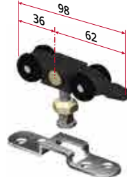
art. 2203 60* Carrello in nylon, regolabile Nylon carriage adjustable
