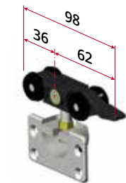
art. 2203/39 160* Carrello in nylon regolabile completo di staffa art. 2239 Nylon carriage adjustable with metal bracket art. 2239
