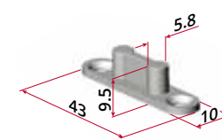
art. 4006 Pattino guida inferiore in nylon Nylon lower guide
