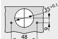
For screw fixing
