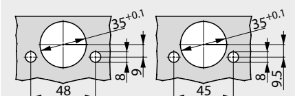
Combination drilling pattern for Impresso
