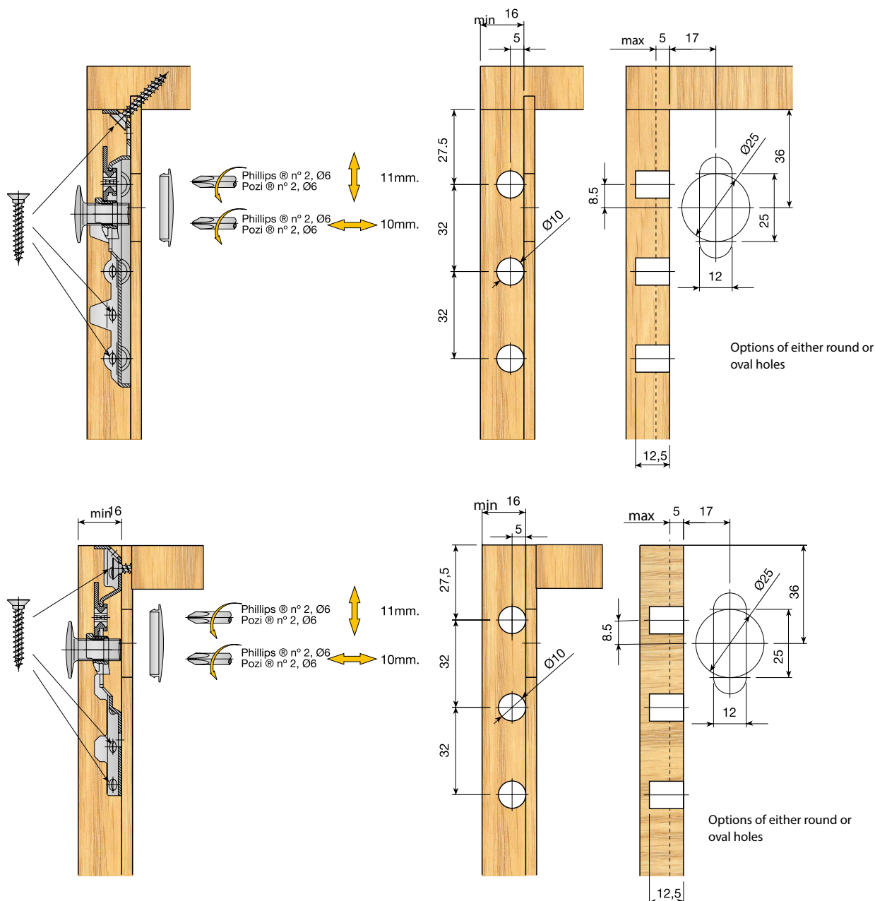
Assembly on to a cabinet with a deep top
