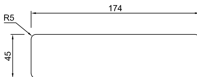
dima foro / hole template
