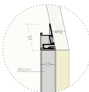
FBS7554 + FBS2063 (decoro decor)
