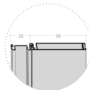
FBS7547 + FBS2010 (maniglia handle)
