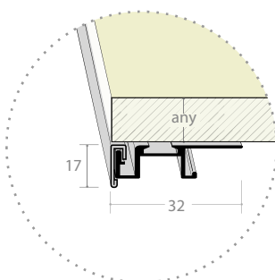
FBS7554 + FBS2063 (decoro decor)
