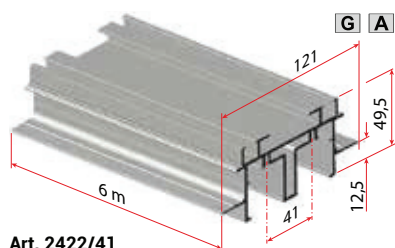
Art. 2422/41
