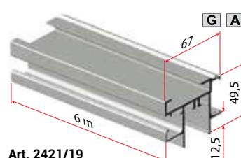
Art. 2421/19
