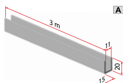
Art. 5824/A
